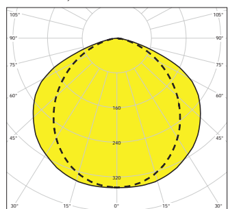
SALUKA-N-LED, IP66
