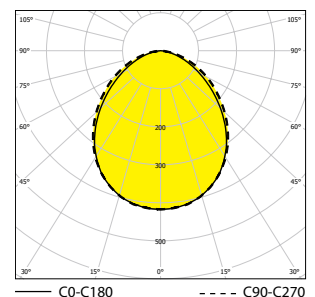
SALUKA-LED-PLUS/FROST-OP
