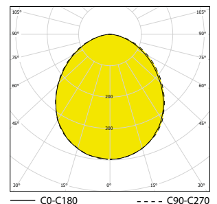
EXTREME-LED-PLUS/FROST-OP
